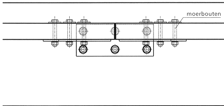
Detail 0602 houten windverband
